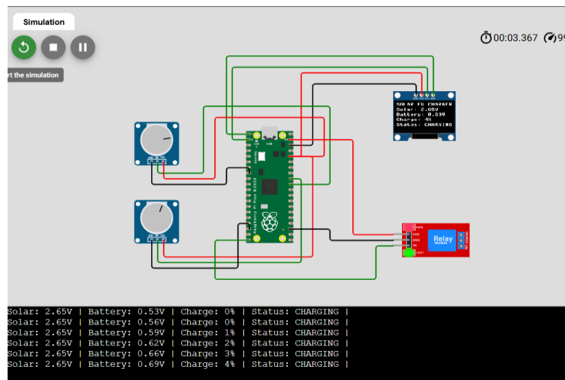
Fig. 3. Circuit Diagram
