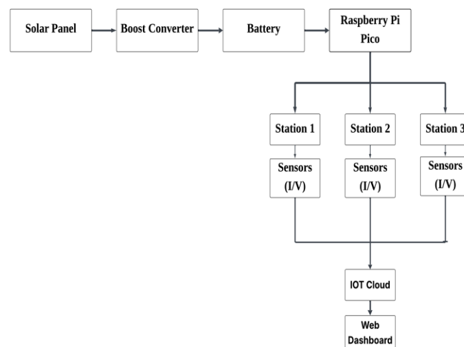
Fig. 2. Three-Node Architecture
