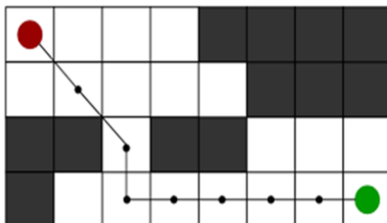
Figure 3. A* Algorithm
