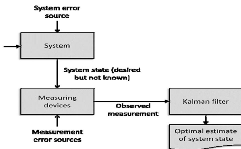
Figure 2. Kalman Filter
