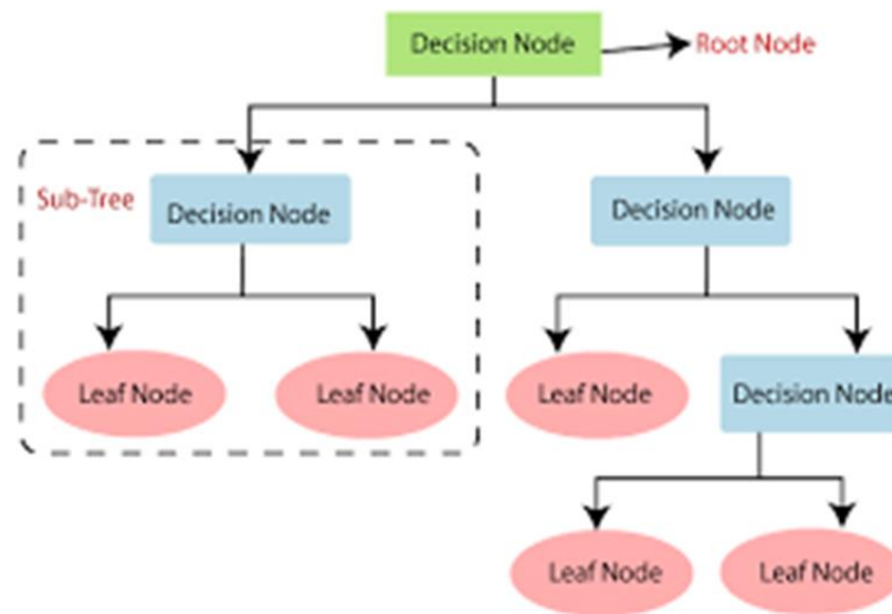
Figure 4. Decision Tree
