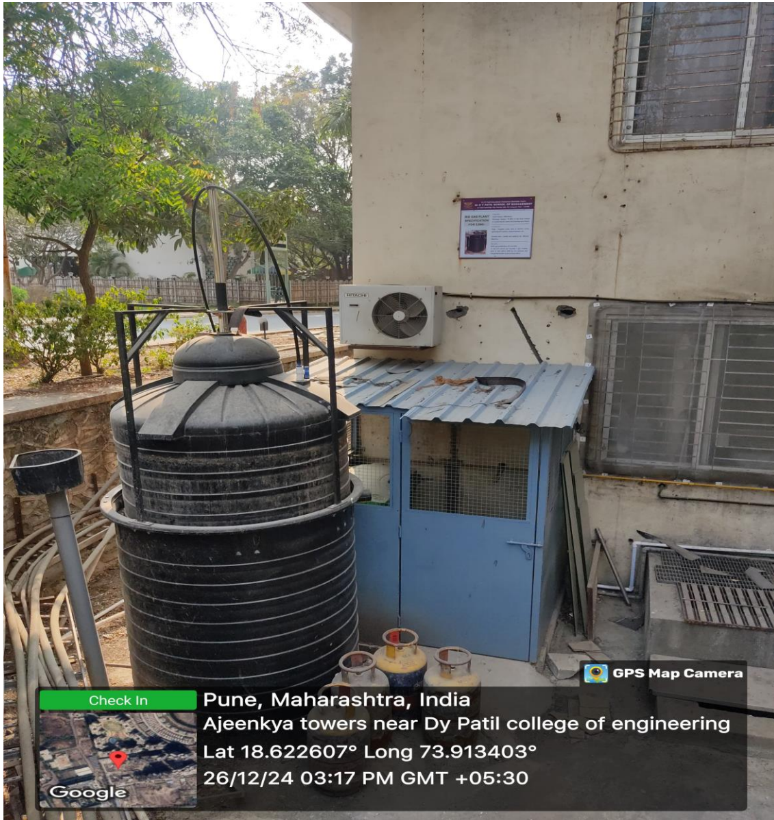
Biogas Plant.
