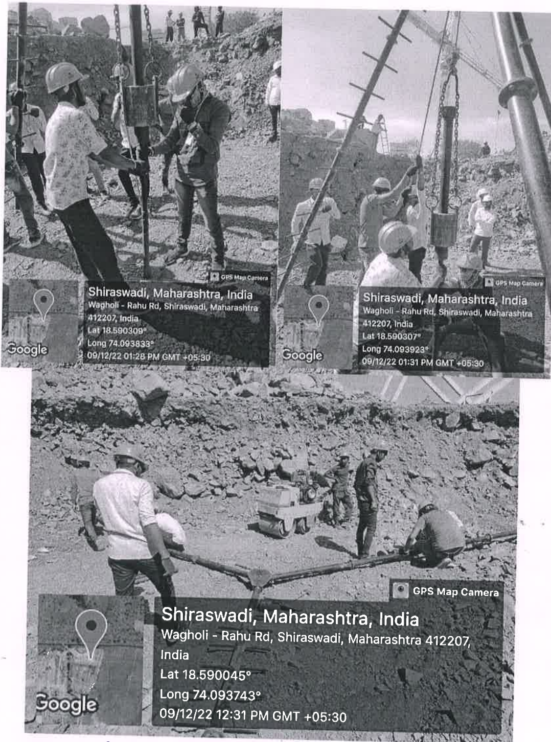
Photo:- Prof Gayatri. C. Sherkar conducting SPT test on soil at Shiraswadi
