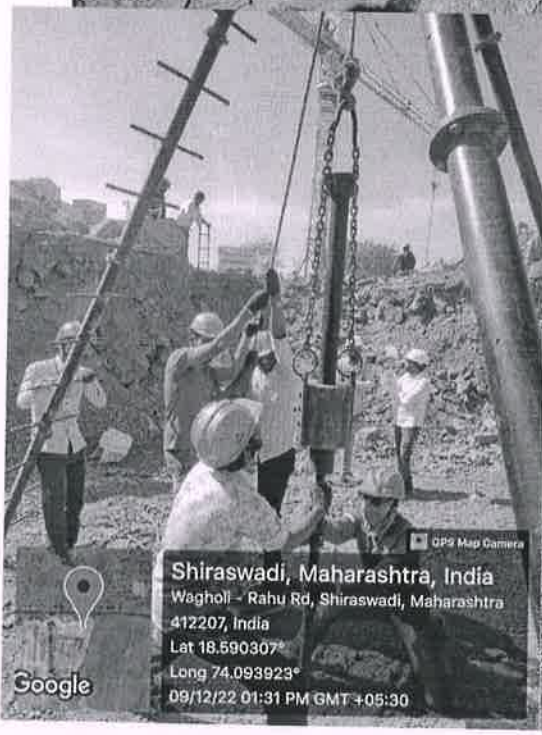
Photo : Alligning & setting up SPT Test apparatus at site
